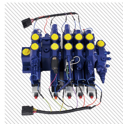
垃圾压缩车阀 Refuse compression collector valve XGHW-PL138-D5-3
