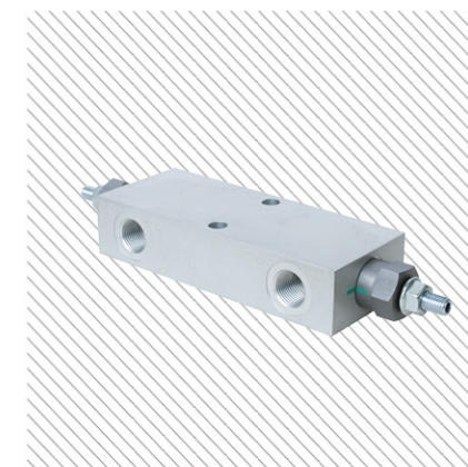
平衡阀 Balance valve DCB60-35A-4.25
